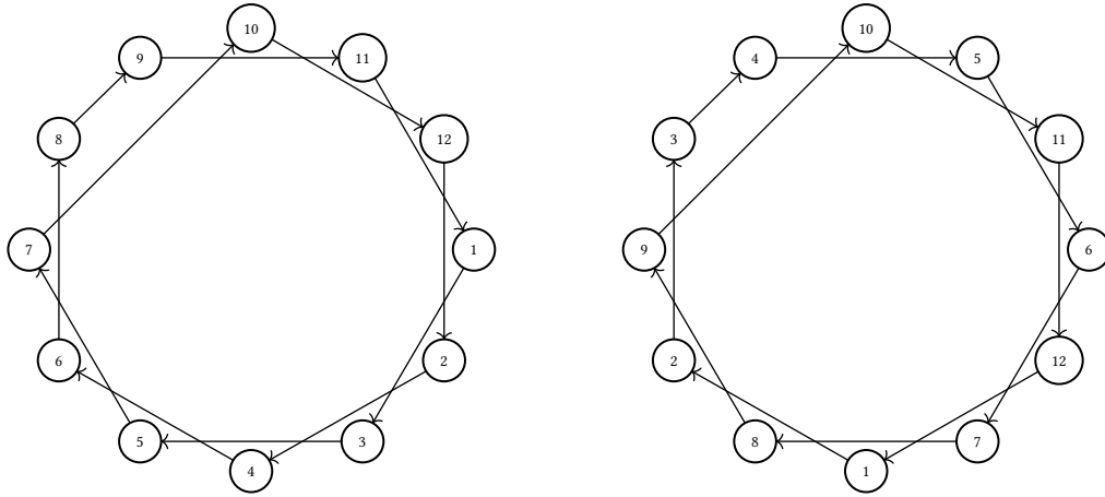
Figure 2: G : Two isomorphic directed graphs due to the function f ,
